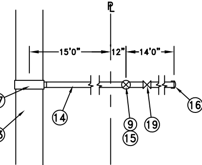
PRESSURE SEWER LATERAL
