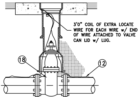
PAVED AREA LOCATE WIRE TERMINATION
