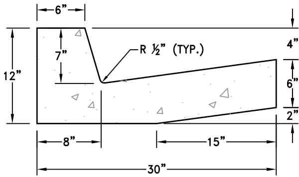
30" CURB & GUTTER – TYPE A 0.57 YD. 3 /10 LINEAR FT. N.T.S.
