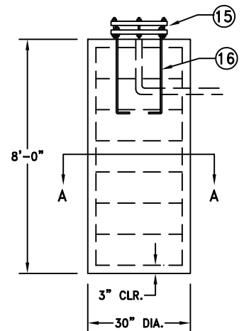
SLIP BASE
