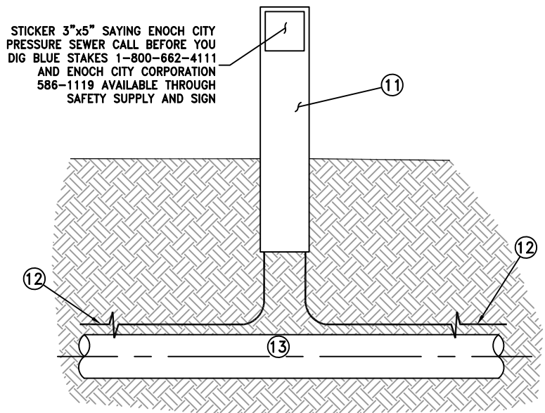
UNPAVED AREA LOCATOR POST DETAIL
