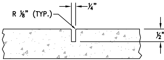
CONNECTION JOINT N.T.S.
