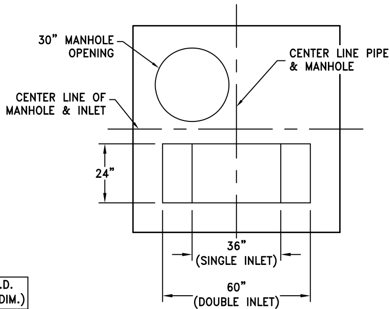
CURB INLET CUT-OUT DETAIL N.T.S.
