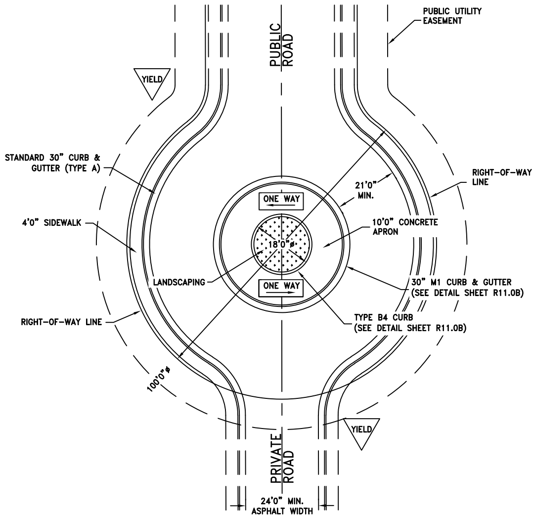
P.U.D. ACCESS TURN-AROUND PLAN VIEW N.T.S.
