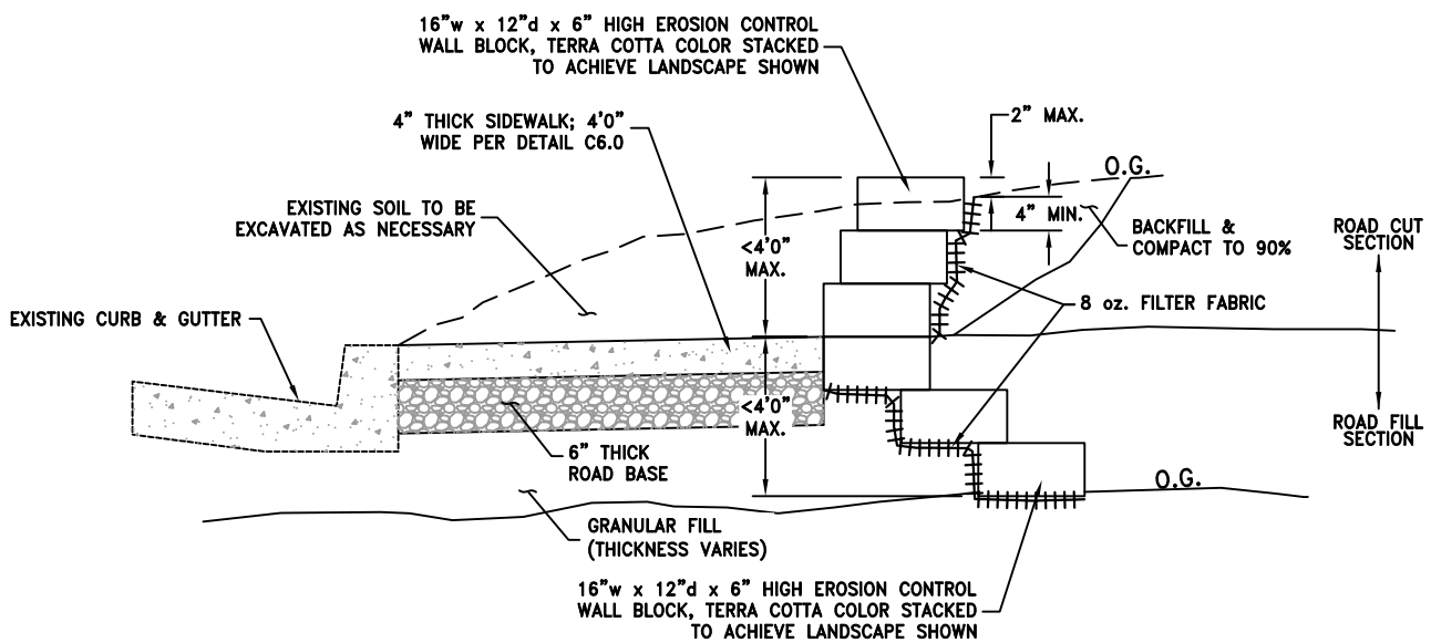
EROSION CONTROL WALL @ BACK OF SIDEWALK N.T.S.
