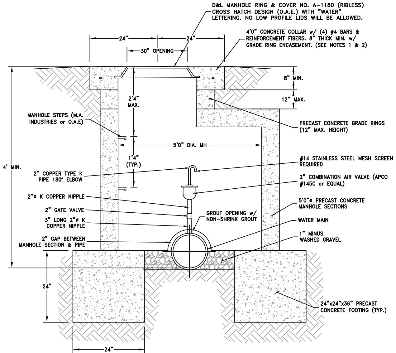
COMBINATION AIR VALVE DETAIL IN ROADWAY
