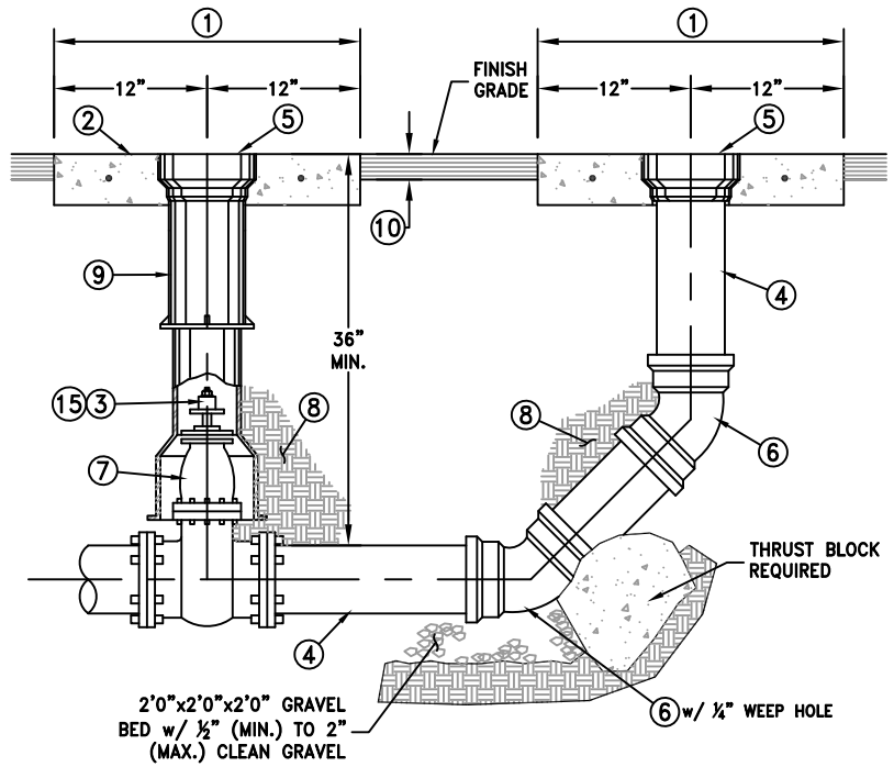
PRESSURE SEWER CLEAN-OUT DETAIL
