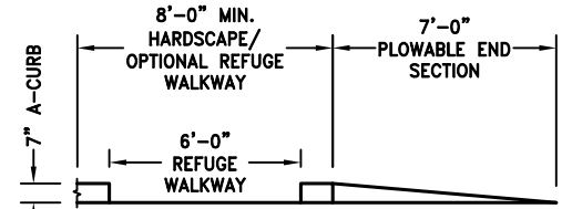
WALKWAY & PLOWABLE END PROFILE
