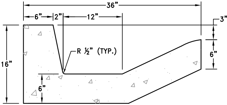
36" CURB & GUTTER – TYPE C 0.81 YD. 3 /10 LINEAR FT. N.T.S.
