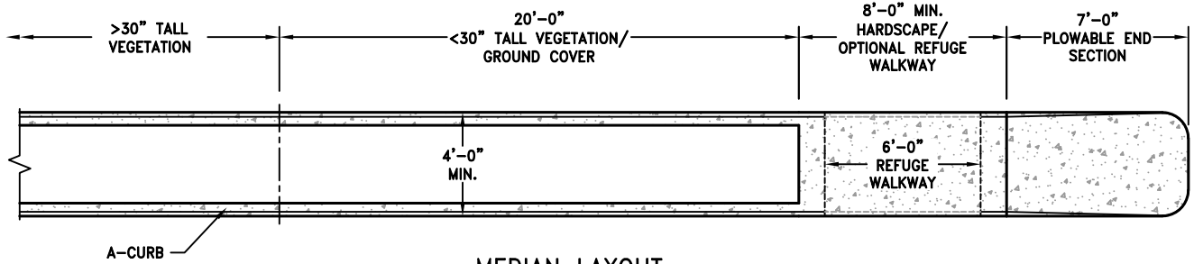
MEDIAN LAYOUT
