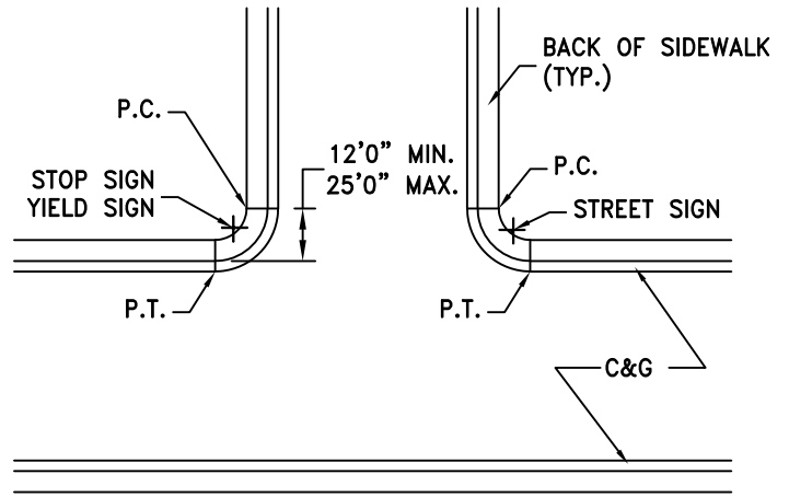
STOP & STREET SIGN LOCATION DETAIL N.T.S.
