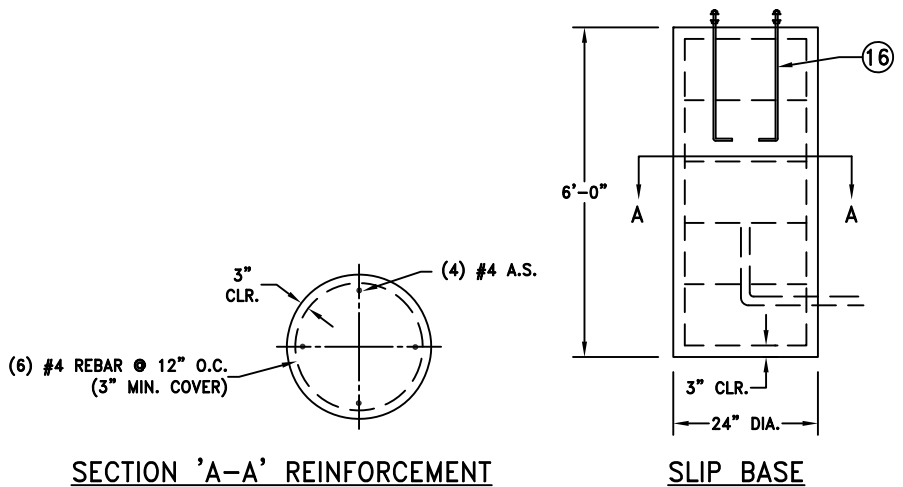
LIGHT POLE FOUNDATION DETAIL N.T.S.
