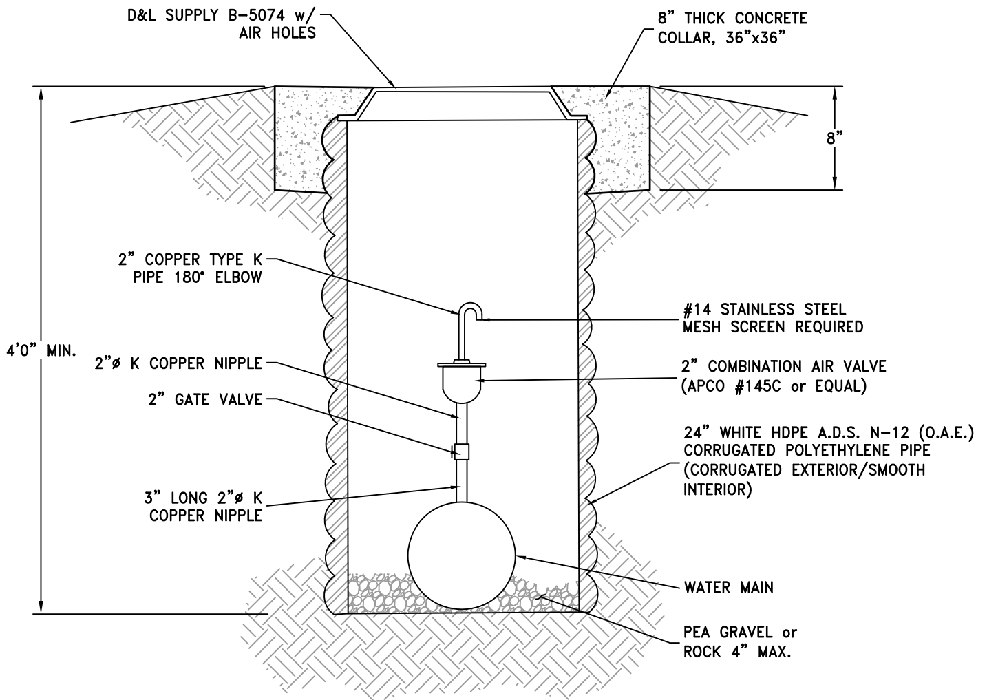
COMBINATION AIR VALVE DETAIL OUTSIDE ROADWAY
