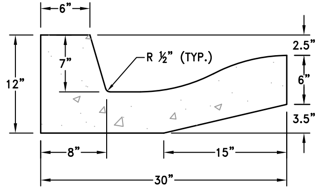
30" IRRIGATION CURB & GUTTER – TYPE B 0.57 YD. 3 /10 LINEAR FT. N.T.S.
