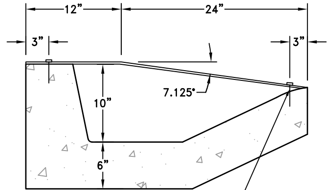
1/2" x 4" ANCHOR BOLT (GALVANIZED) w/ 5/8" HOLE (SPACED 2' O/C & ON ALL CORNERS)
